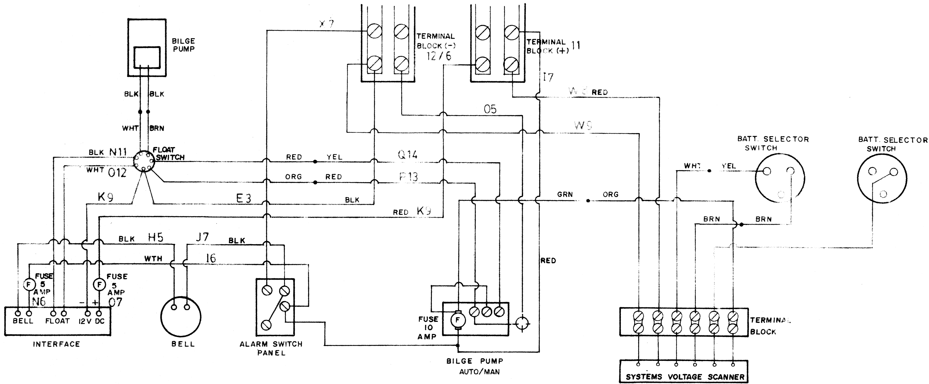
BILGE PUMP & HIGHWATER ALARM WIRING DIAGRAM
